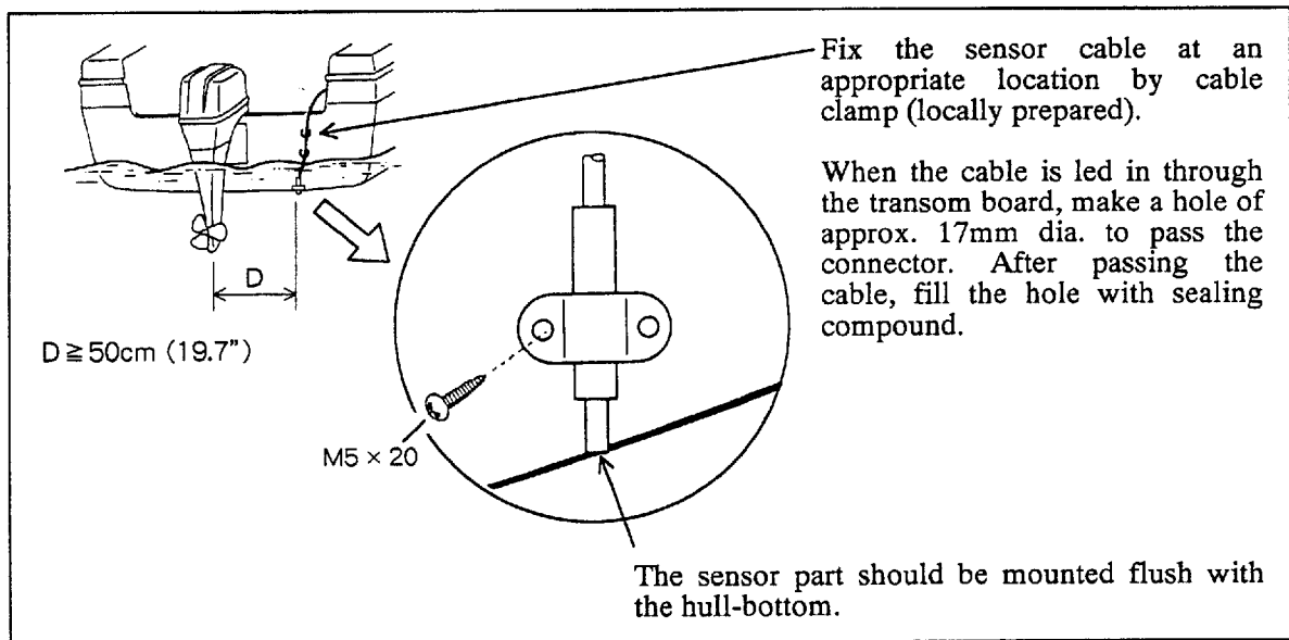
Figure 11 How to mount transom mount temperature sensor
